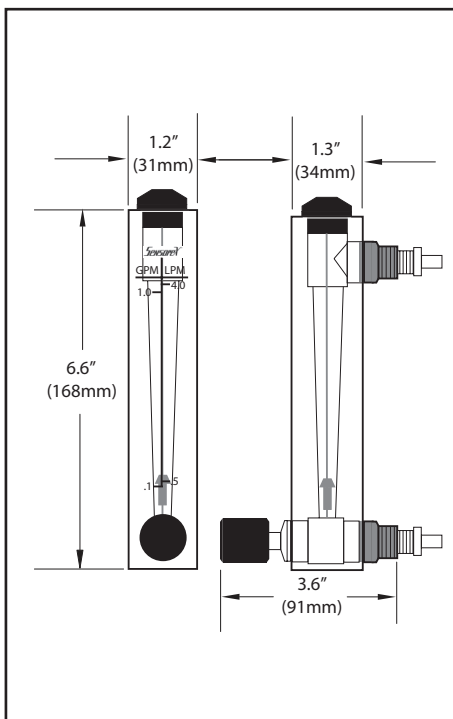
FLOW METER FM001 DIMENSIONS
